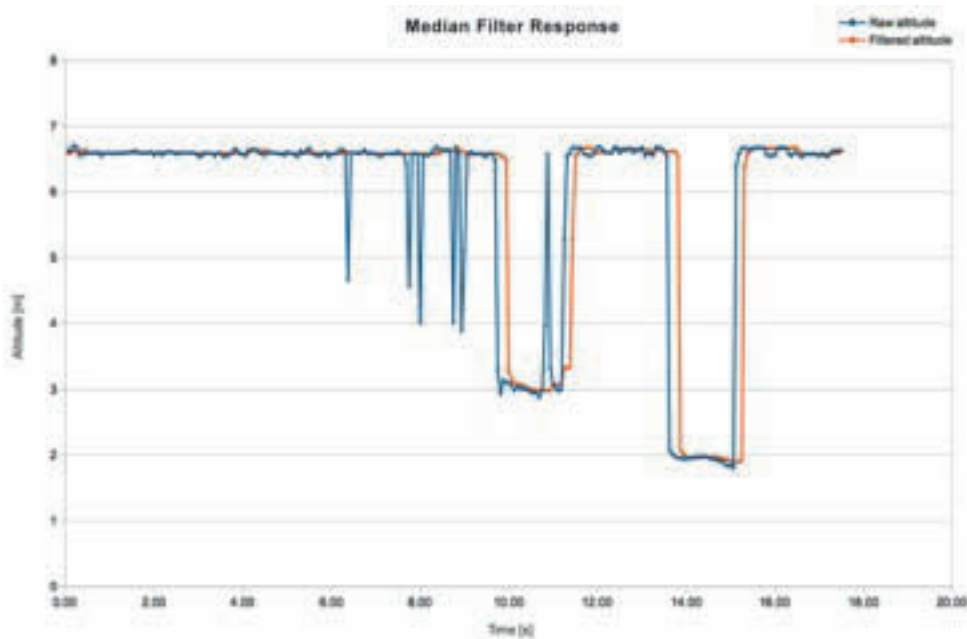
Figure 11 :: Median Filter Response graph
