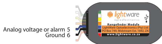
Figure 5 :: Analog voltage connections
